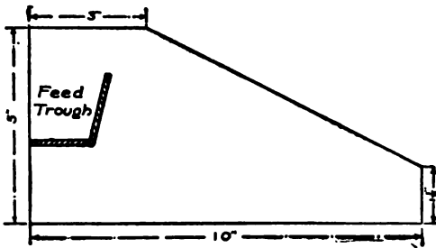
FIG. 241. — Stall Partitions.
